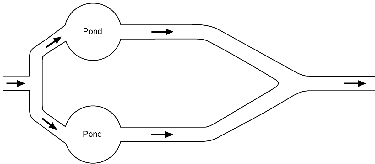
Figure 5.13-3 Parallel ponds allow continued treatment of storm water during pond maintenance.
